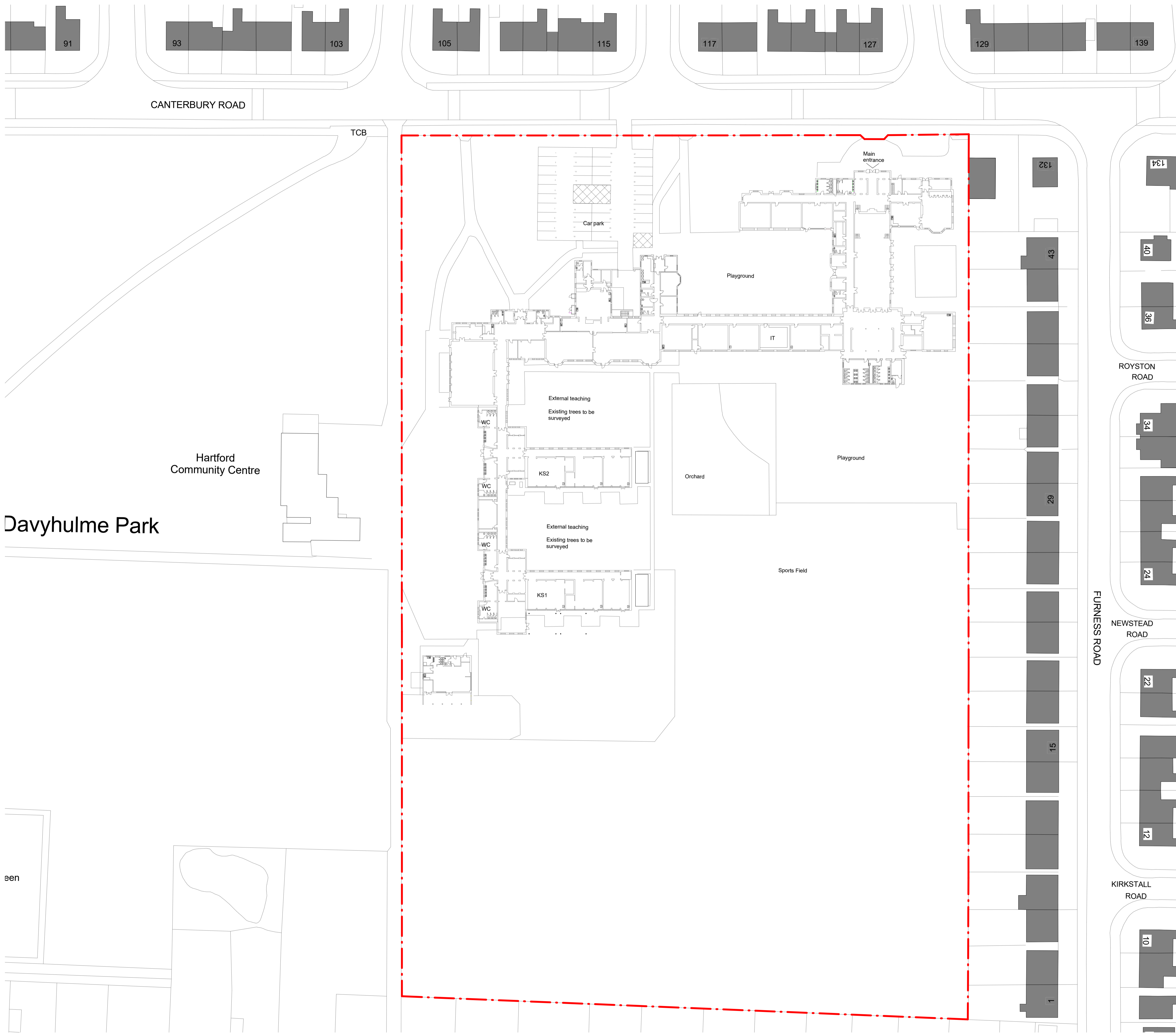
1 Existing Site Plan 1 : 500 @ A1
